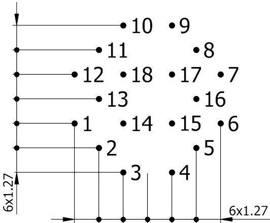
Recommended PCB Layout PCB Top View
