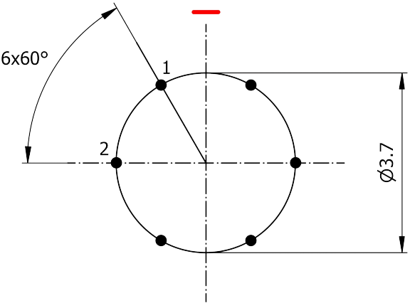
Recommended PCB Layout PCB Top View
