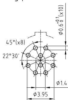
PCB drilling pattern
