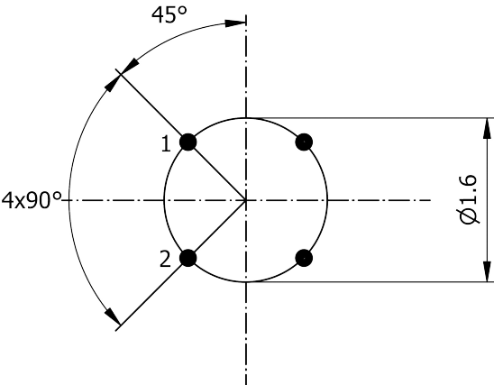
Recommended PCB Layout PCB Top View
