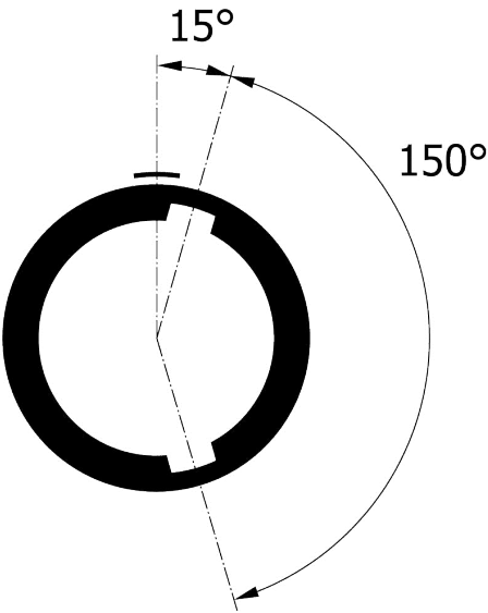
Alignment Key Front View
