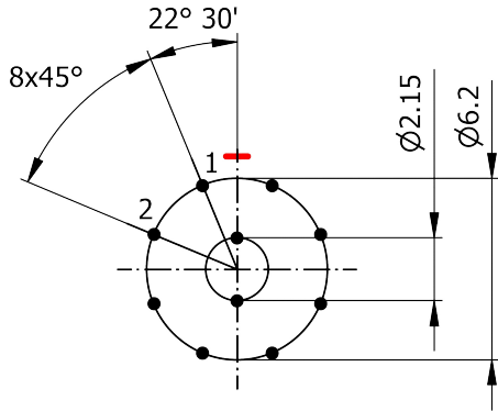
Recommended PCB Layout PCB Top View
