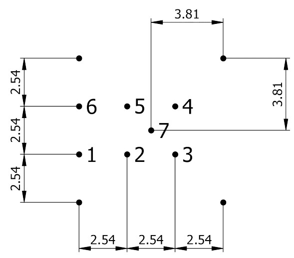
Recommended PCB Layout PCB Top View
