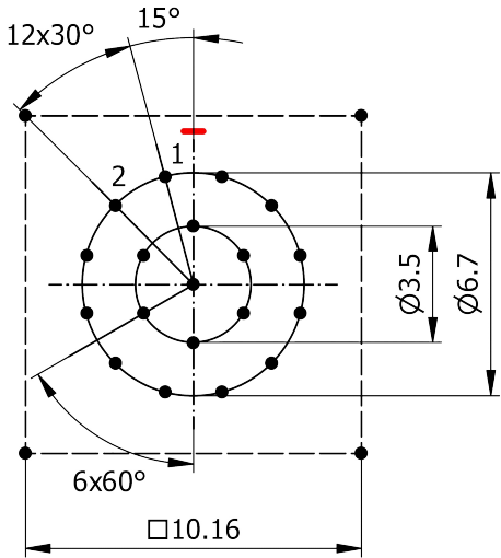
Recommended PCB Layout PCB Top View
