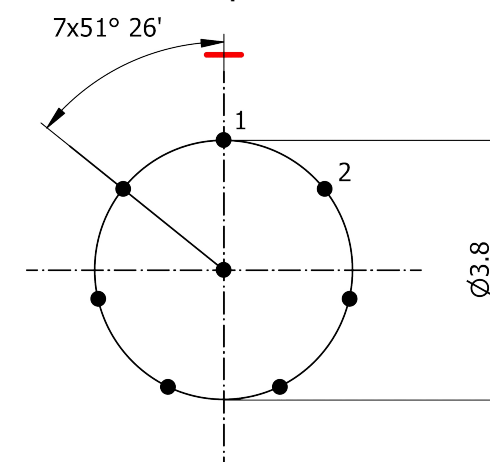
Recommended PCB Layout PCB Top View
