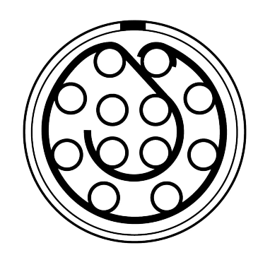
Insert Configuration Rear View
