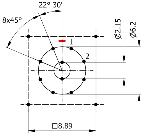
Recommended PCB Layout PCB Top View
