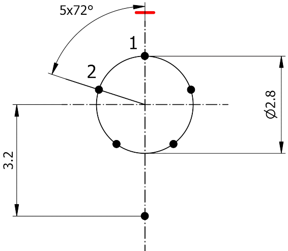
1) Recommended PCB Layout PCB Top View
