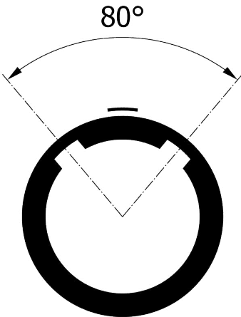
Alignment Key Front View
