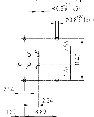
A-A cross-section (PCB drilling pattern)
