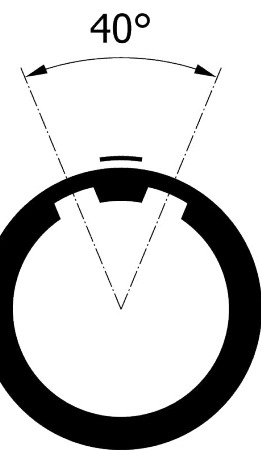
Alignment Key Front View
