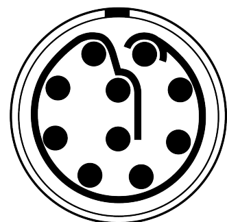
Insert Configuration Front View
